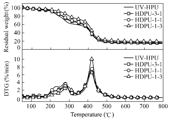
图 11 TG (a) and DTG (b) curves of UV-HPUA and DHPUA coatings
