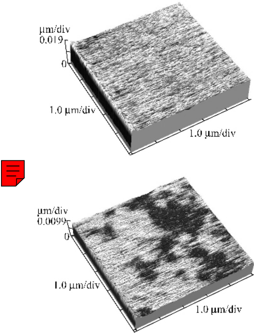
Fig. 3 Surface topography of UV-HPUA coatings before and after moisture cure
