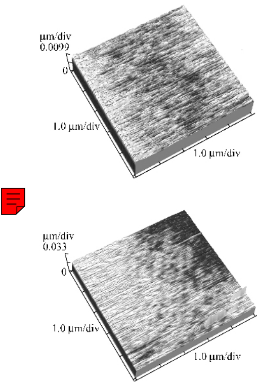
Fig. 7 Surface topography of DHPUA-1-1 coatings before and after moisture cure
