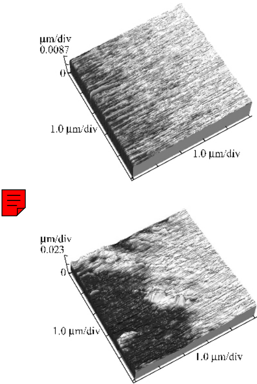
Fig. 8 Surface hist ogram of DHPUA-1-1 coatings before and after moisture cure
