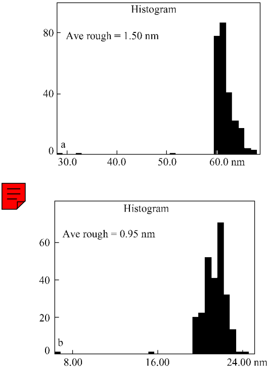
Fig. 6 Surface histogram of DHPUA-3-1 coatings before and after moisture cure
