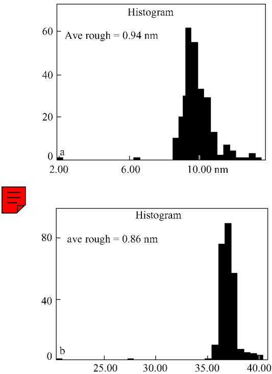
Fig. 8 Surface hist ogram of DHPUA-1-1 coatings before and after moisture cure
