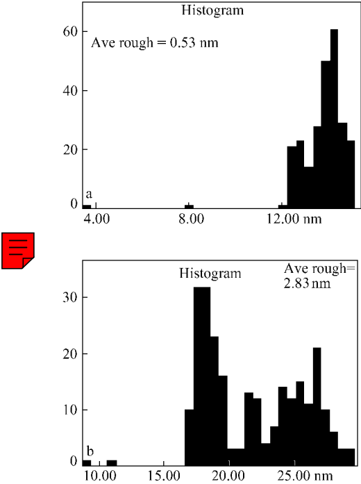
Fig. 10 Surface histogram of DHPUA-1-3 coatings before and after moisture cure
